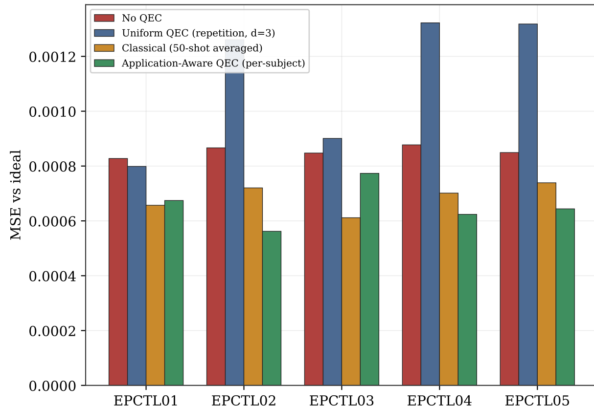
MSE vs ideal, per subject (seed-averaged)
