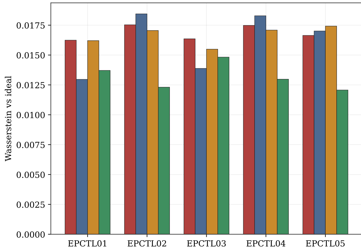
Wasserstein vs ideal, per subject (seed-averaged)
