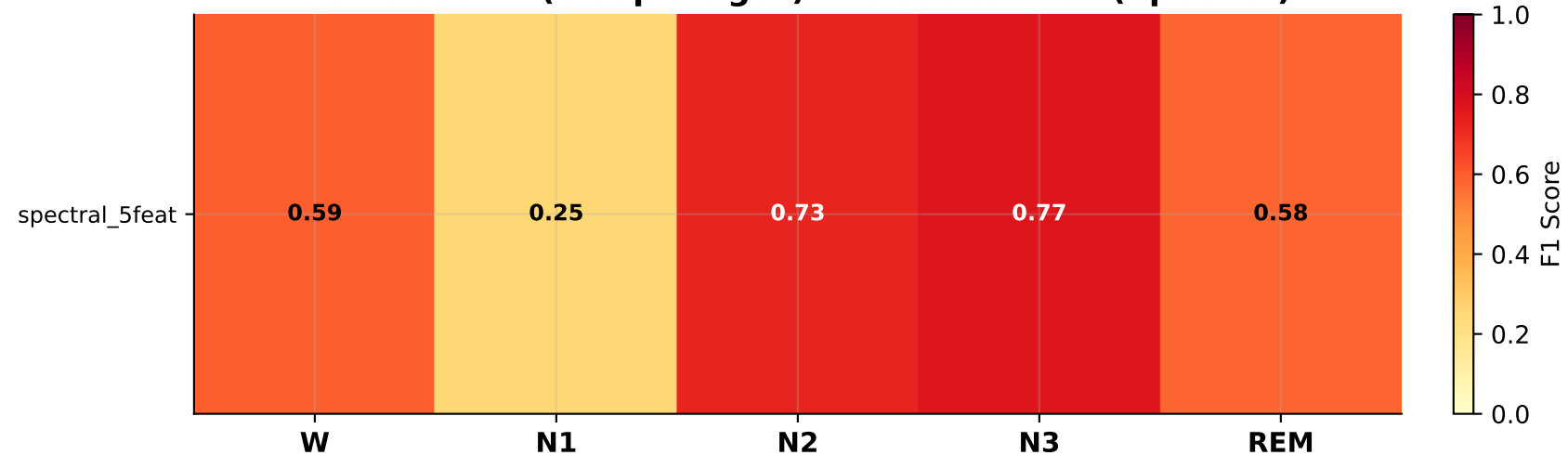
Per-Class F1 (Sleep Stages) — Classical BCE (Spectral)
