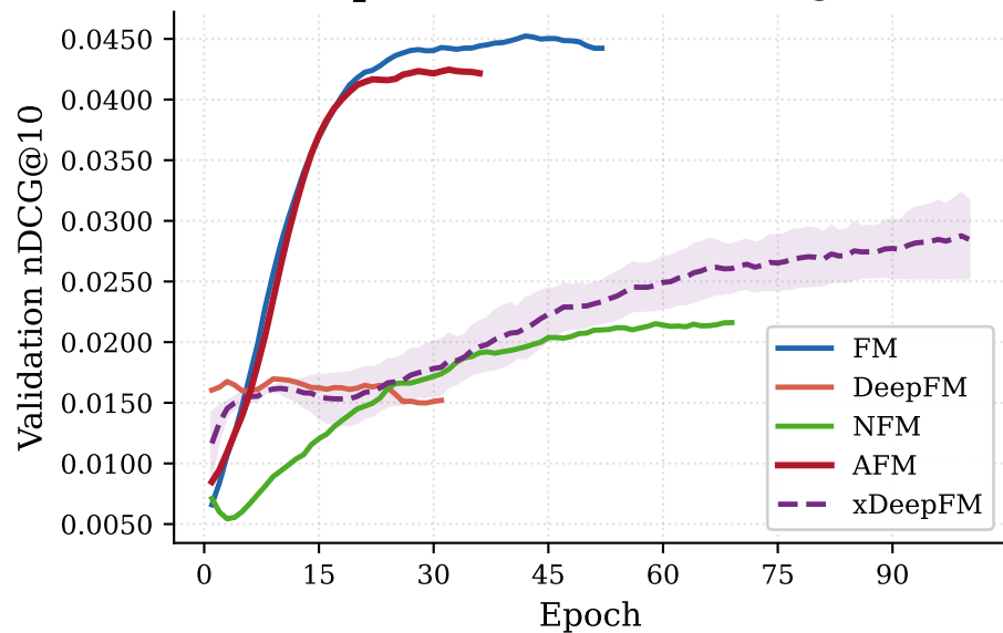
Yelp — Validation nDCG@10
