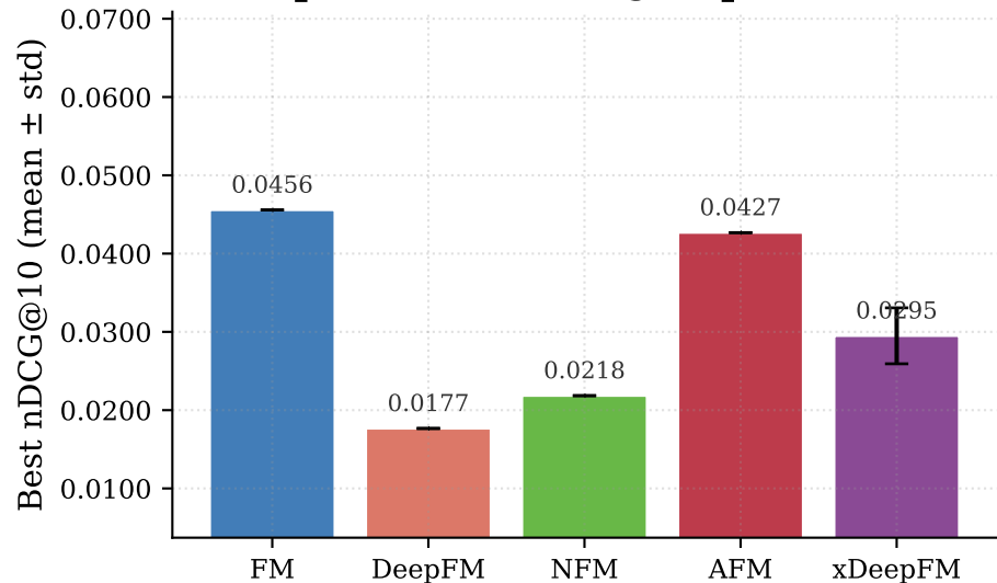
Yelp — Best nDCG@10 per Model
