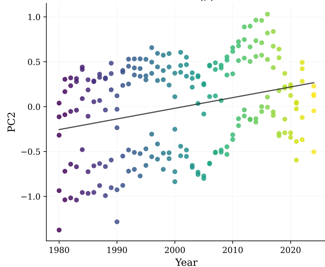
Years vs PC2 ( |\rho|=0.27 )
