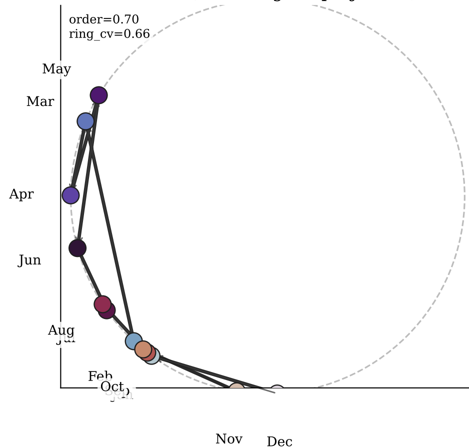
Months (order-aligned projection)
