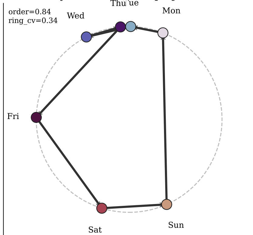
Days (order-aligned projection)
