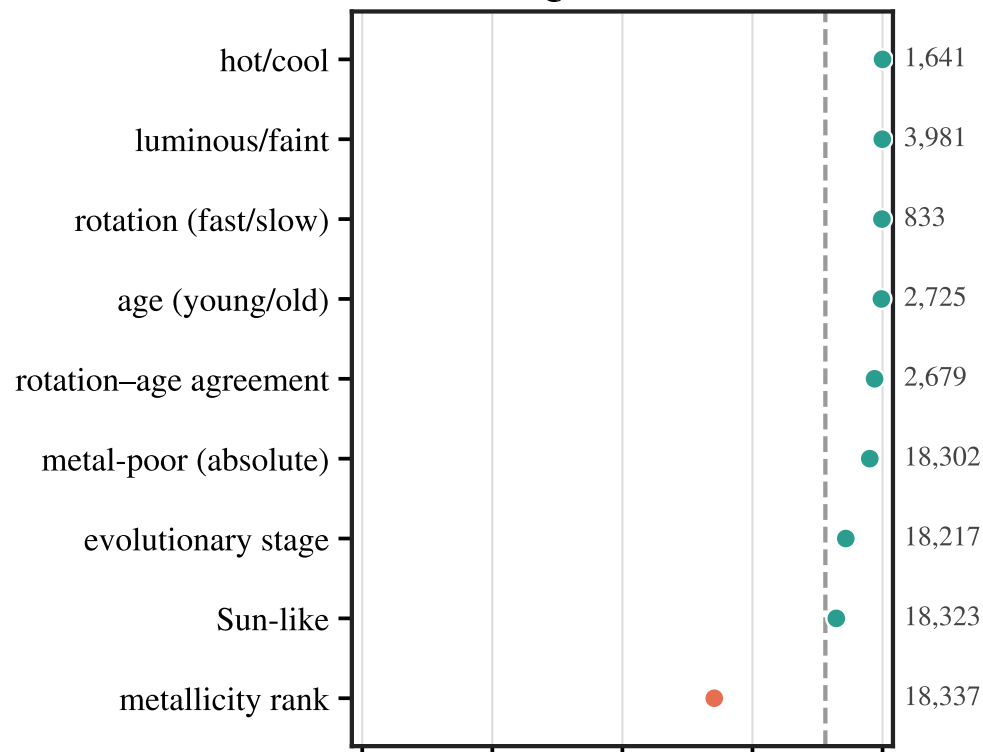
Qualitative
