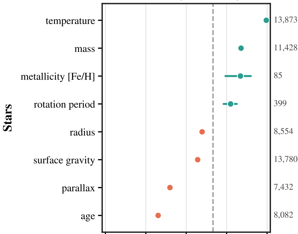
Numeric (within 10%)
