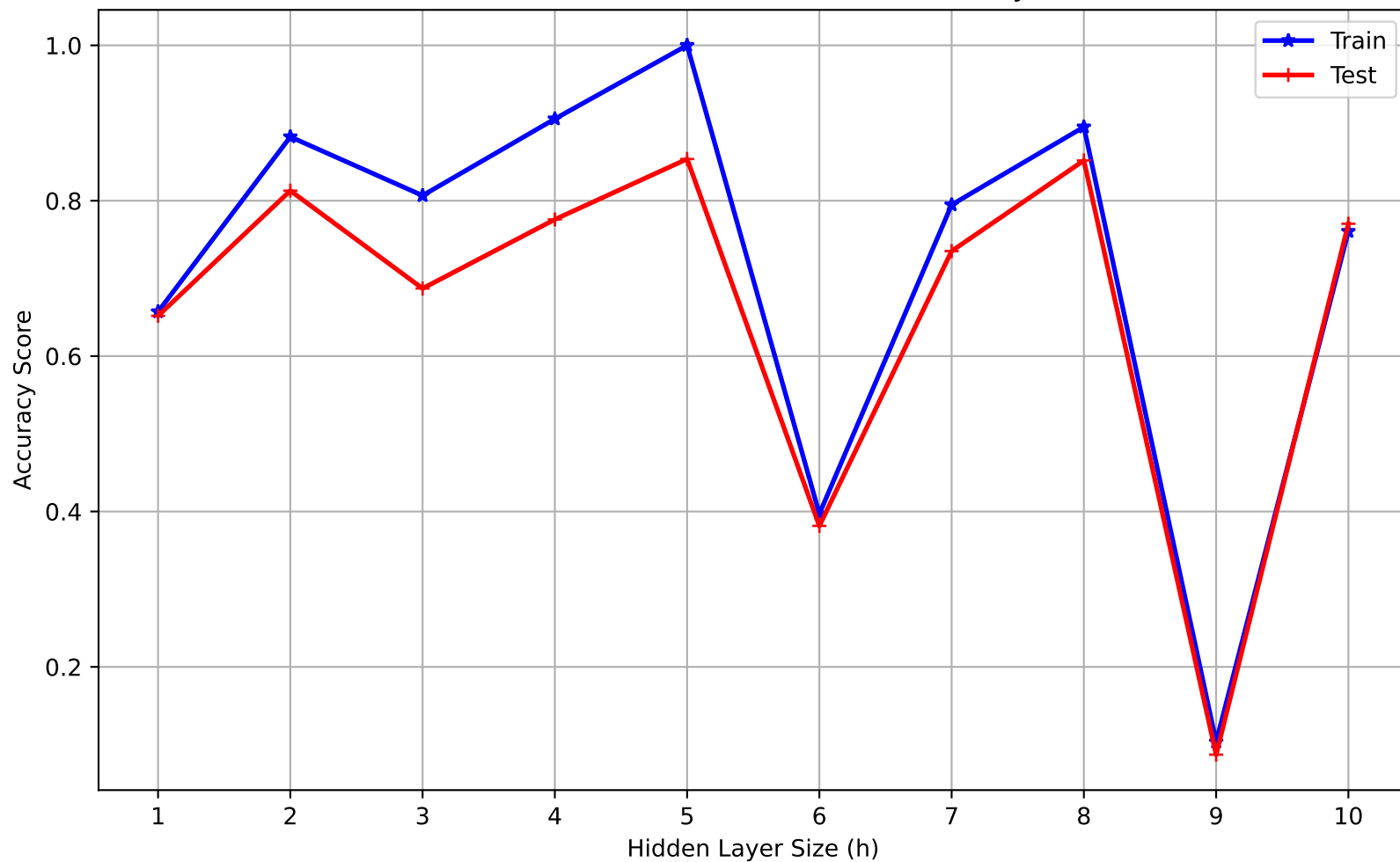
Train & test scores as a function of hidden layer size
