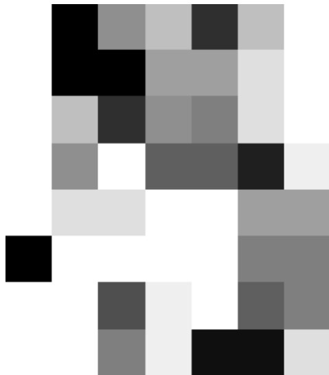
Noisy ( |x-16| )
