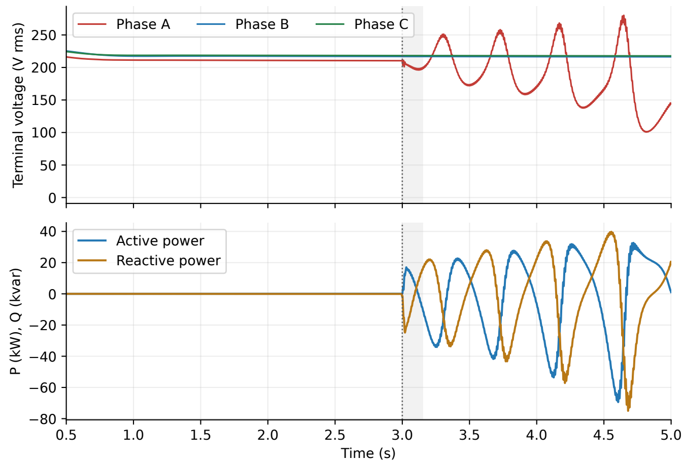
Remote inverter connection at 3.0 s
