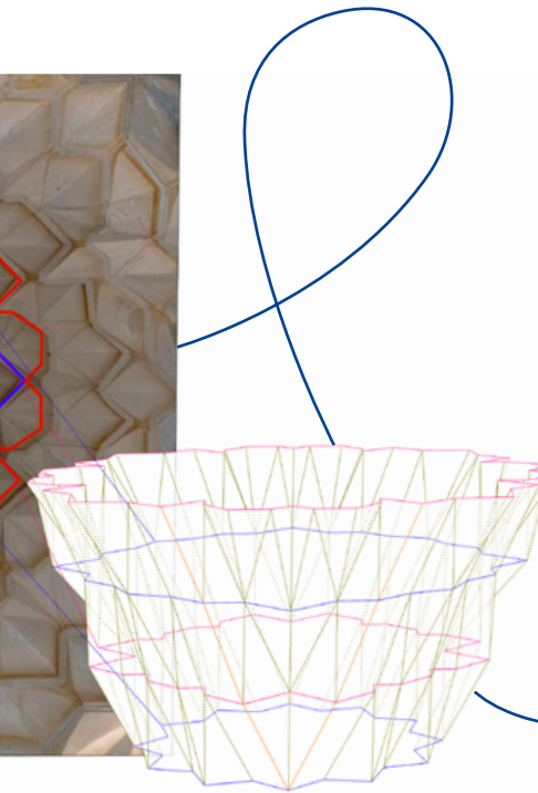
Analyzing and constructing the pattern of the tomb for a plaster-mold
