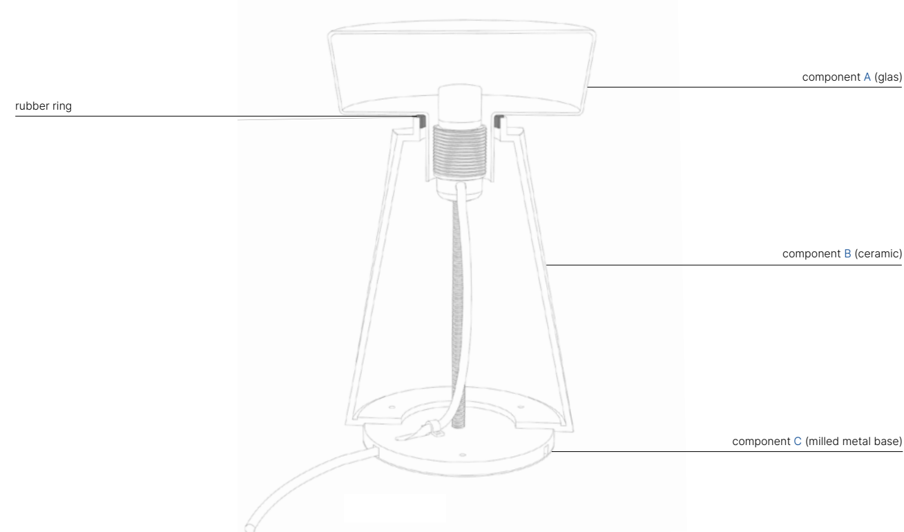
Technical drawing, Side-cut
