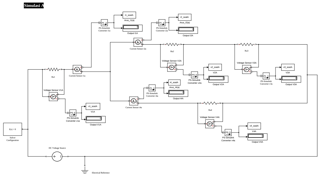
Figure 3.1. model_tugas3/Rangkaian Soal A
