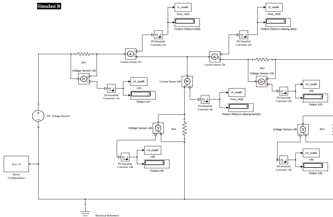
Figure 3.2. model_tugas3/Rangkaian Soal B
