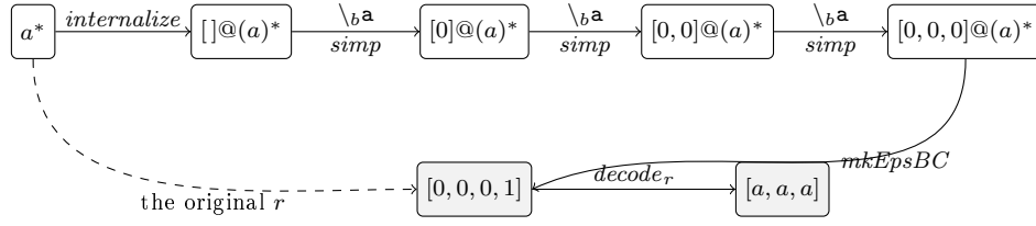
Figure 5.6: The bit-coded construction on a^* against "aaa". Every arrow between expressions points forward, and no ri_i is needed once its successor exists. The expression stays two nodes wide while the bit-prefix grows by one 0 per iteration. The dashed arrow is the one backward dependency left: decode needs the original r to know what shape the bits describe.
