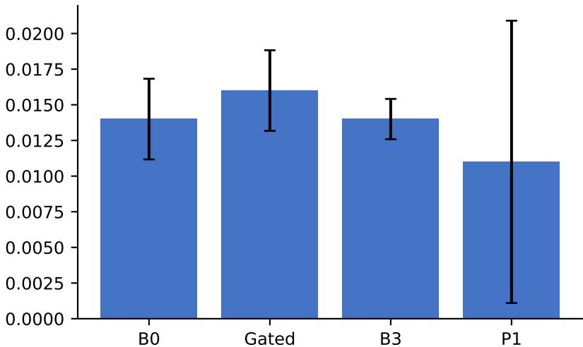
Exact accuracy
