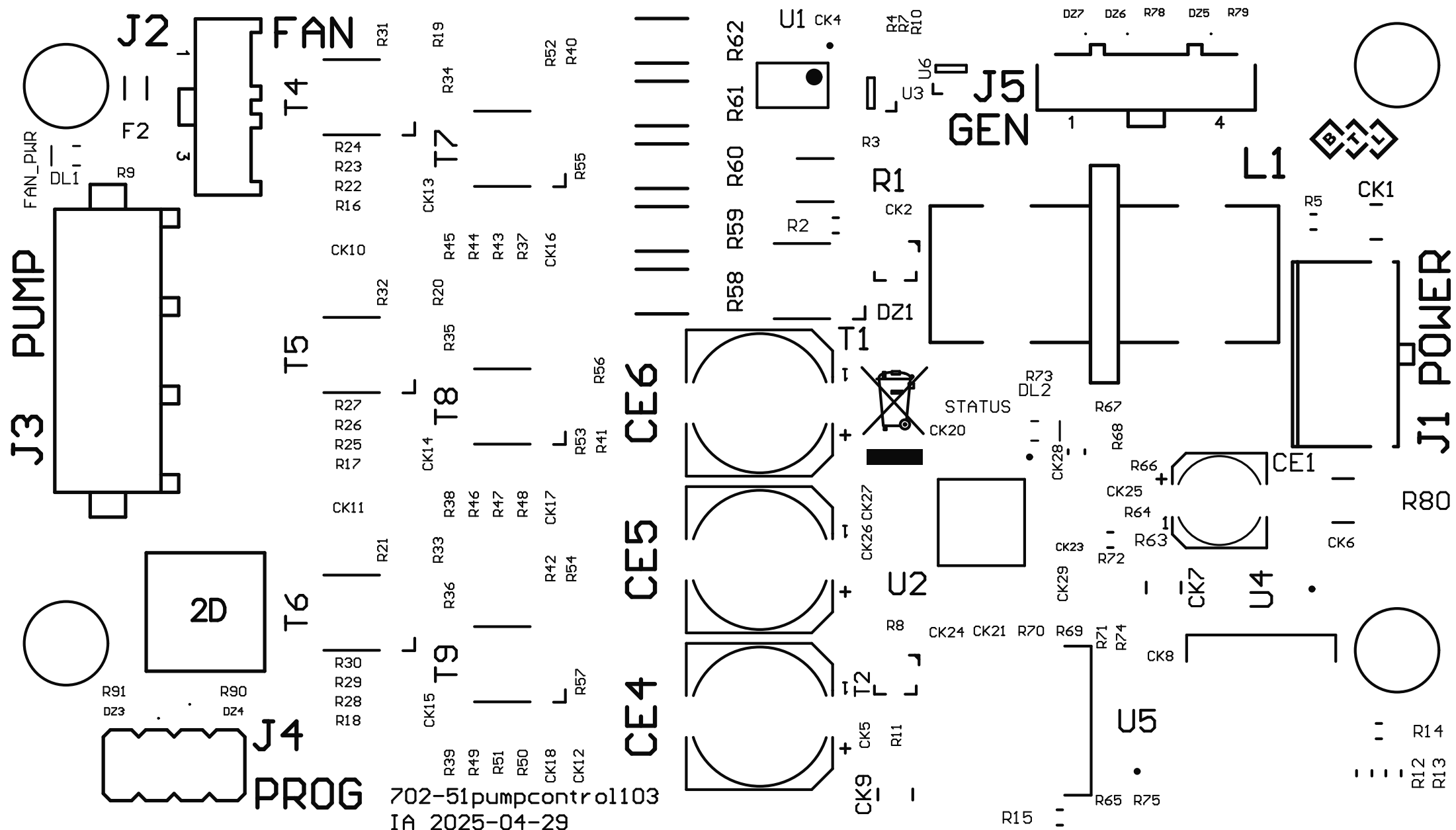
Top Silkscreen
