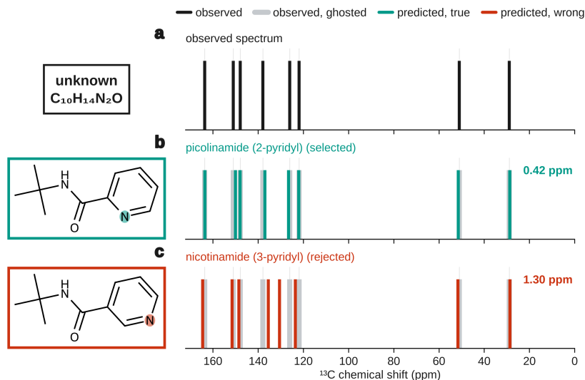
Figure S5: Locked v3-R25 verify-save (main-text Figure 5). Self-rank prefers 3-pyridyl; forward ^{13}\text{C} recovers 2-pyridyl (chamfer 0.42 vs 1.30 ppm). A verify-save, not a recall win. Not Listing 1.
