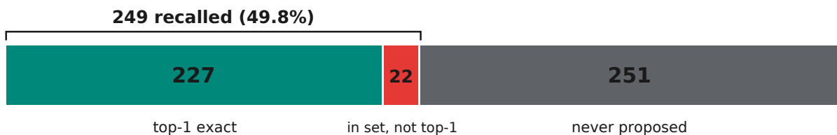
Figure S3: Reprint of the n=500 generation wall (fig_wall_diagnostic): 227 top-1 exact / 22 in set but not top-1 / 251 never proposed. Same integers as Figure S1. Propose is the wall, not verify.
