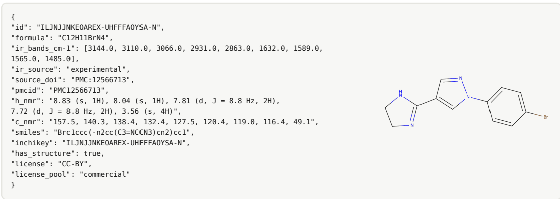
Figure S2: Reprint of main-text Listing 1 (listing1_irexp_record). IReXp JSON+molecule (C 12 H 11 BrN 4 ; ILJNJNKEOAREX-UHFFFAOYSA-N). SMILES and InChIKey are resource fields, not solver payload.
