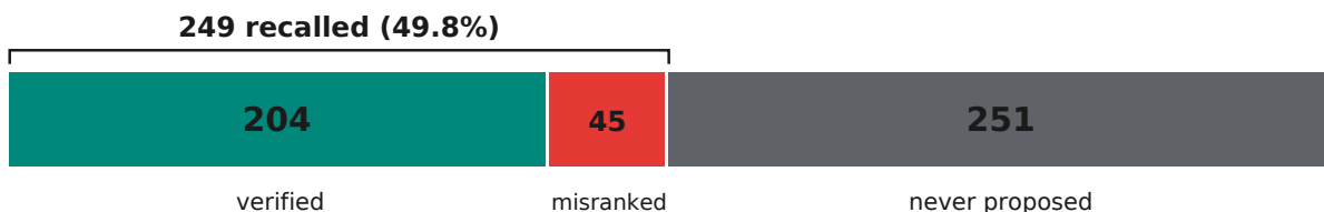
Figure S3: Reprint of the n=500 forward-verify wall (fig_wall_diagnostic): 204 verified / 45 misranked / 251 never proposed. Source: spectro-agent data/fverify_n500/WALL_n500.md. Generation remains 227/500 top-1 and 249/500 recall.
