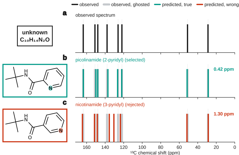
Figure S4: Locked v3-R25 verify-save (main-text Figure 5). Self-rank prefers 3-pyridyl; forward ^{13}C recovers 2-pyridyl (chamfer 0.42 vs 1.30 ppm).
