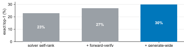
Figure S4: Inference ladder on the 60-compound arm: 23% \rightarrow 27% \rightarrow 30% (generate-wide recall 32% \rightarrow 42%). Moved from the main text; integers unchanged.
