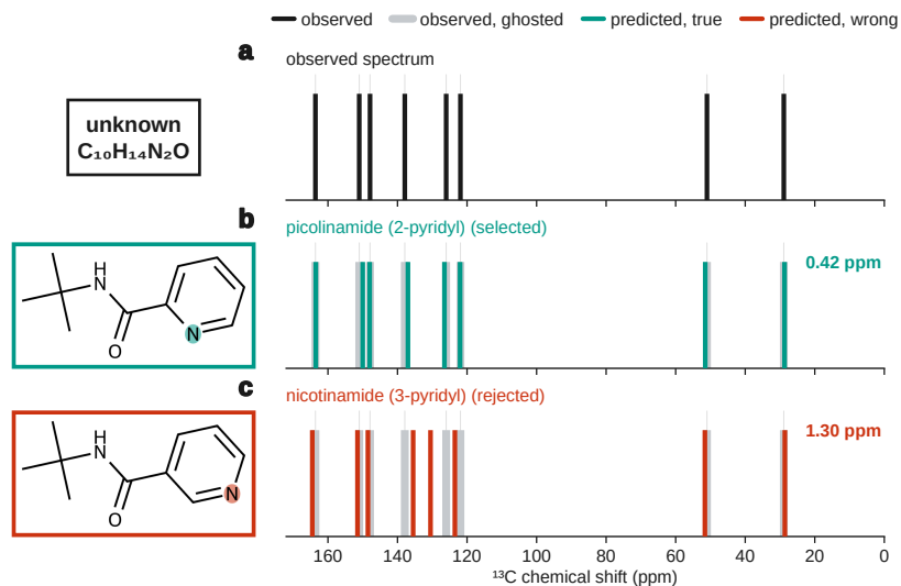
Figure S5: Case v3-R25 shows a verify-save (main-text Figure 3): self-rank prefers 3-pyridyl, while forward ^{13}\text{C} recovers 2-pyridyl (chamfer 0.42 vs 1.30 ppm).
