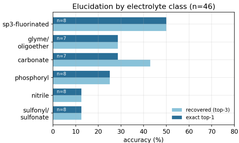
Fig. S3: IRSpectra-Bench-Electrolyte by battery-electrolyte class (n=46): \text{sp}^3\text{-C-F} easiest (50%), sulfonyl and nitrile hardest (12%).
