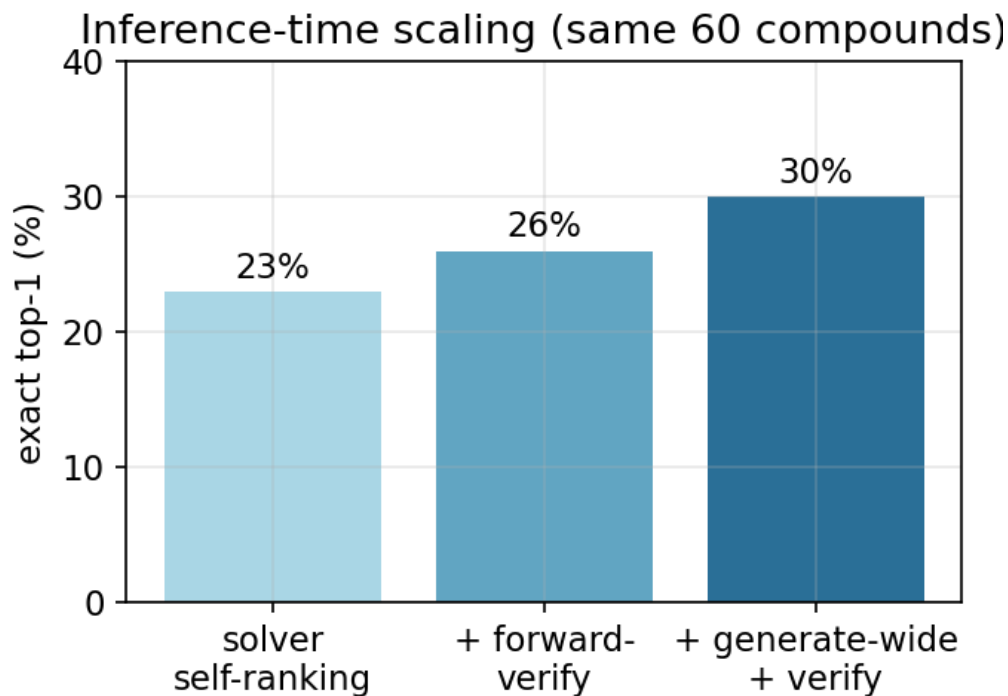
Fig. 5: Forward-verification inference ladder on the same 60 compounds: solver self-ranking \rightarrow + forward-verify \rightarrow + generate-wide (23%/26%/30% top-1).
