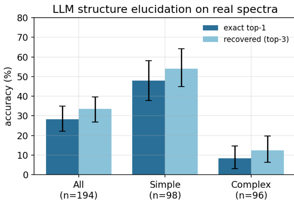
Fig. 2: Top-1 and recovered accuracy on IRSpectra-Bench by difficulty (all / simple / complex, n=194) with bootstrap 95% CIs.
