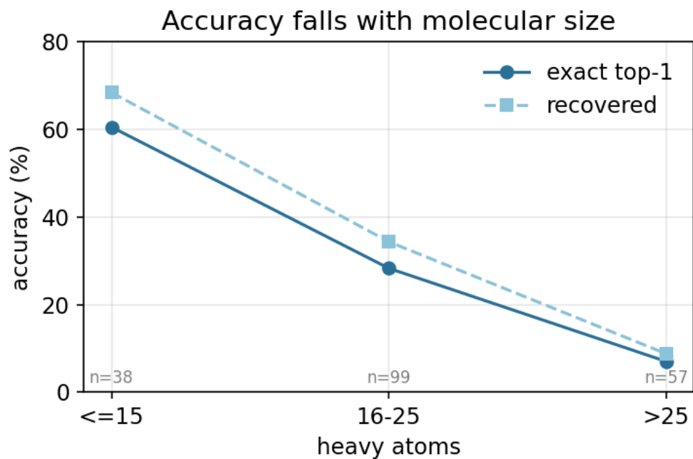
Fig. S2: Accuracy versus molecular size; the monotonic 60% \rightarrow 7% top-1 gradient with heavy-atom count.
