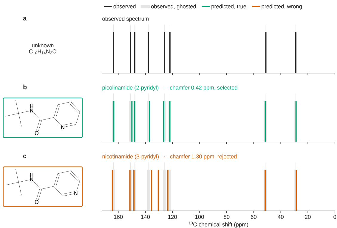
Fig. 6. Forward-verification on a benchmark regioisomer pair: picolinamide and nicotinamide are indistinguishable to the inverse task, but the true isomer’s forward-predicted 13 C spectrum matches the observed one at a chamfer of 0.42 ppm against 1.30 ppm for the alternative (§5.1).
