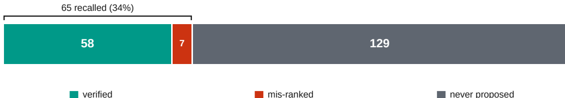
Fig. 1. Diagnosis on IRSpectra-Bench ( n=194 ): generation recall, not verification, is the bottleneck. Where the true structure is proposed, forward-verification ranks it first 89% of the time (58/65); where it is never proposed (66% of the bar), no ranker can recover it. End-to-end top-1 is the product of those two rates ( \approx 30\% ), which have different denominators and are not differenced.
