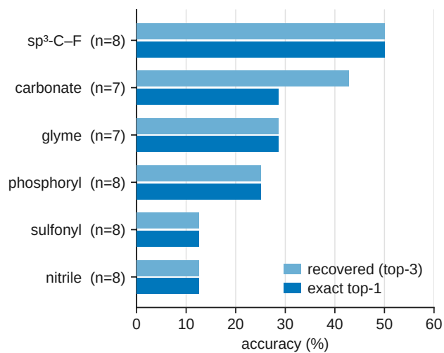
Fig. S4. IR Spectra-Bench-Electrolyte by battery-electrolyte class (n=46).
