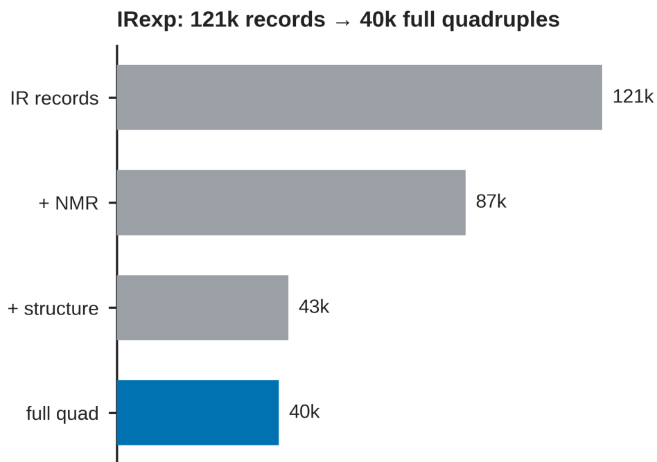
Fig. S1: IRexp composition: IR records, NMR-paired, structure-linked, and full IR+ ^1\text{H} + ^{13}\text{C} +structure quadruples.
