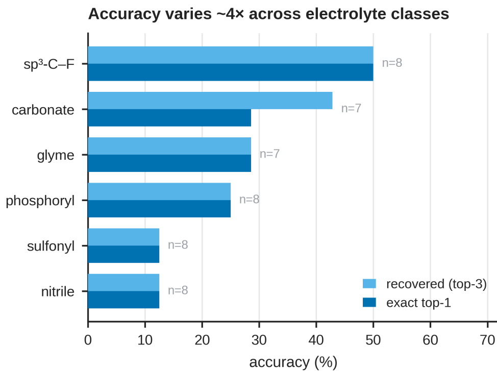
Fig. S3: IRSpectra-Bench-Electrolyte by battery-electrolyte class (n=46): sp 3 -C-F easiest (50%), sulfonyl and nitrile hardest (12%).
