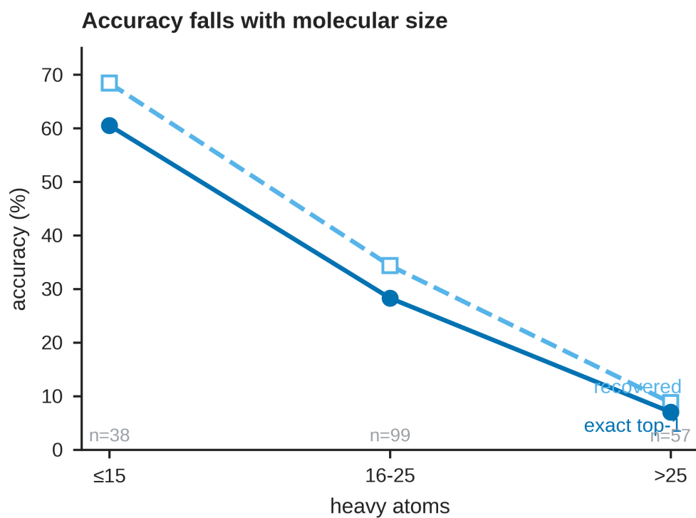
Fig. S2: Accuracy versus molecular size; the monotonic 60% \rightarrow 7% top-1 gradient with heavy-atom count.
