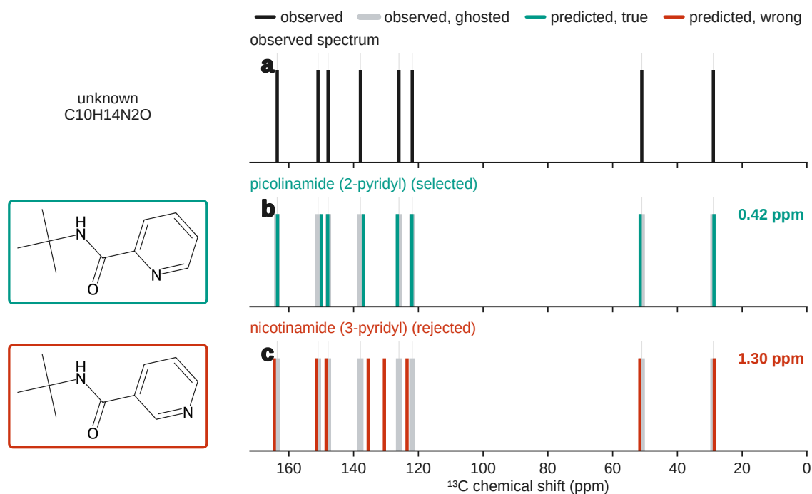
Fig. 6. Forward-verification on a benchmark regioisomer pair: picolinamide and nicotinamide are indistinguishable to the inverse task, but forward-predicted 13 C sticks separate the true isomer from the alternative (§5.1).
