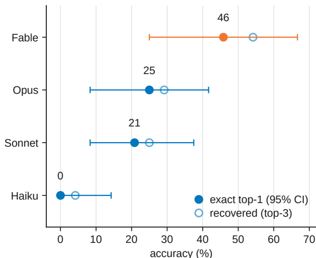
Fig. 3. Four-model comparison on a fixed 24-compound subset, solved blind under one protocol. Outcomes are strictly nested — each stronger model solves a superset of the weaker one’s compounds — so the benchmark is capability-sensitive, but at n=24 it is underpowered to separate adjacent models (§4.4).
