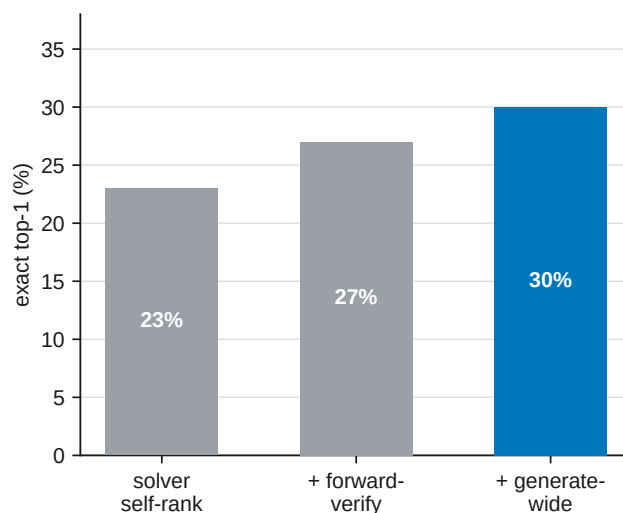
Fig. 7. Forward-verification inference ladder on the 60-compound arm (§5.3). Each stage adds a check on the same compounds; the hero bar is generate-wide top-1.
