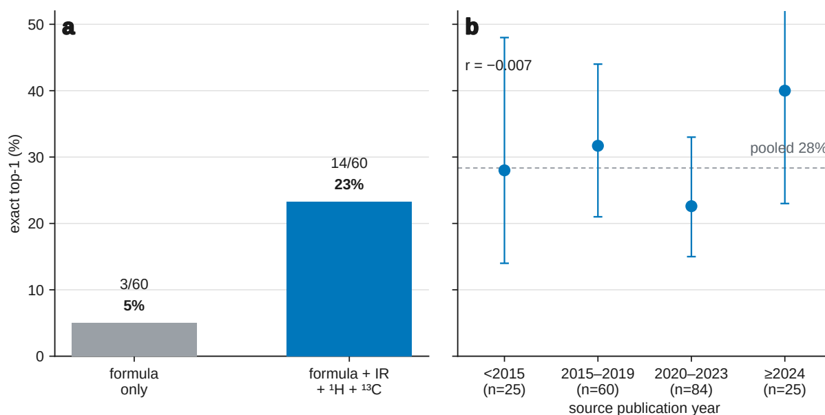
Fig. 4. Two contamination controls. (a) Formula-only vs full modality on 60 compounds. (b) Accuracy vs source-paper year (n=194).
