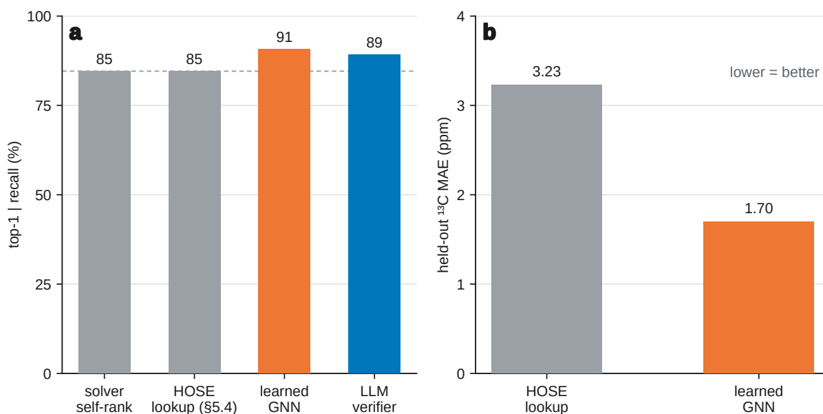
Fig. S6. Learned-verifier probe (§5.4; a complement, not part of the training-free protocol). (a) Conditional-on-recall top-1 over the whole benchmark ( n=65 ) across four verifiers. (b) Held-out ^{13}\text{C} MAE (lower is better).
