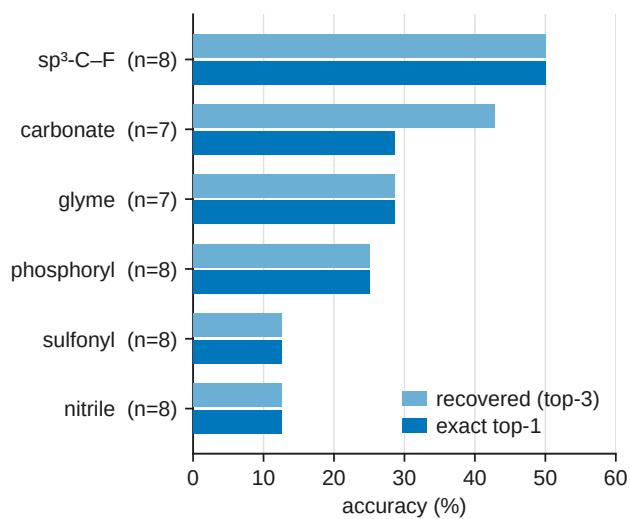
Fig. S4. IRSpectra-Bench-Electrolyte by battery-electrolyte class (n=46).
