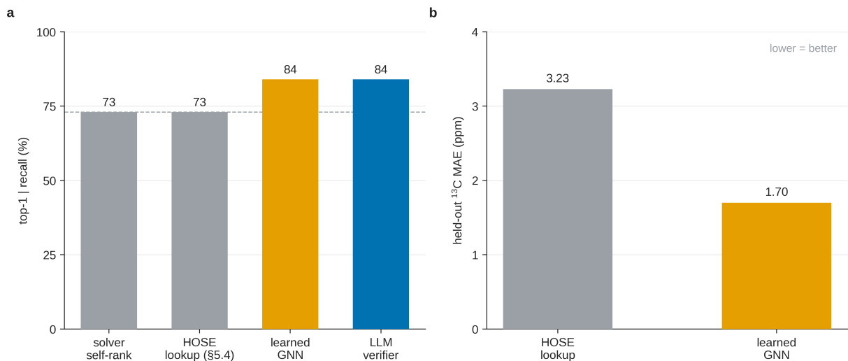
Fig. S6: Learned-verifier probe (§5.7; a complement, not part of the training-free protocol). (A) Conditional-on-recall top-1 (n=19) across four verifiers: a GNN trained on the same nmrshiftdb2 data as the HOSE lookup recovers the LLM verifier’s 84% that the lookup (73%) could not. (B) Held-out 13 C MAE — the learned model is roughly 2× sharper (1.70 vs 3.23 ppm).
