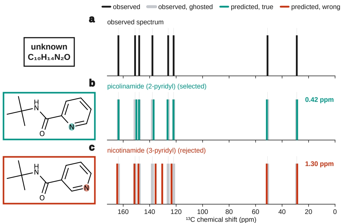
Fig. 6. Forward-verification on a benchmark regioisomer pair: picolinamide and nicotinamide are indistinguishable to the inverse task, but forward-predicted ^{13}C sticks separate the true isomer from the alternative (§5.1).
