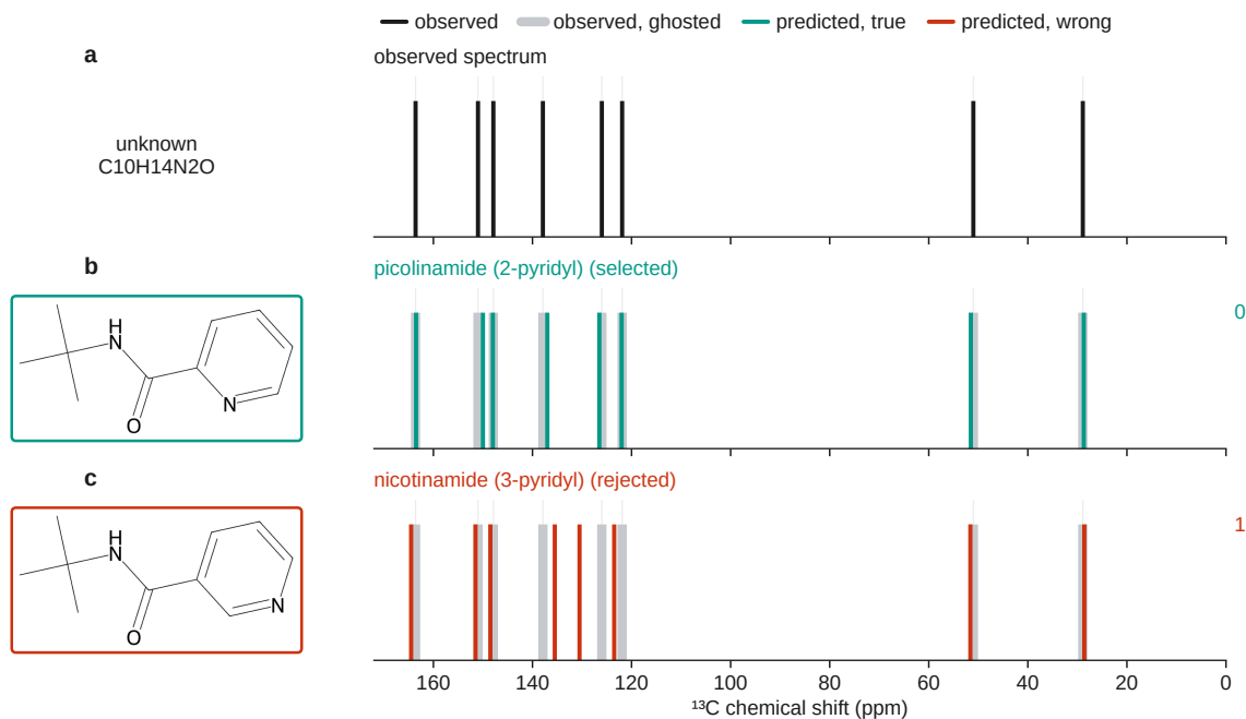
Fig. 6. Forward-verification on a benchmark regioisomer pair: picolinamide and nicotinamide are indistinguishable to the inverse task, but forward-predicted ^{13}C sticks separate the true isomer from the alternative (§5.1).
