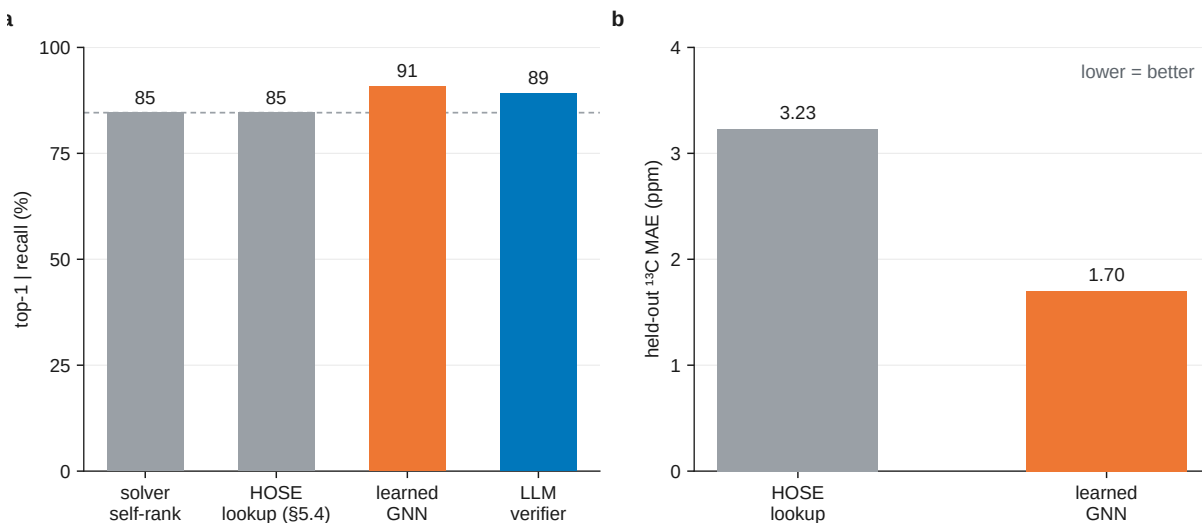
Fig. S6. Learned-verifier probe (§5.4; a complement, not part of the training-free protocol). (a) Conditional-on-recall top-1 over the whole benchmark (n=65) across four verifiers. (b) Held-out 13 C MAE (lower is better).
