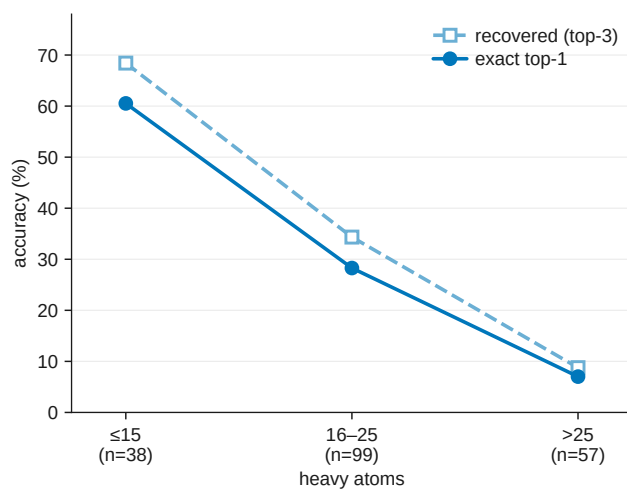
Fig. S3. Accuracy versus molecular size; top-1 falls monotonically as heavy-atom count increases.
