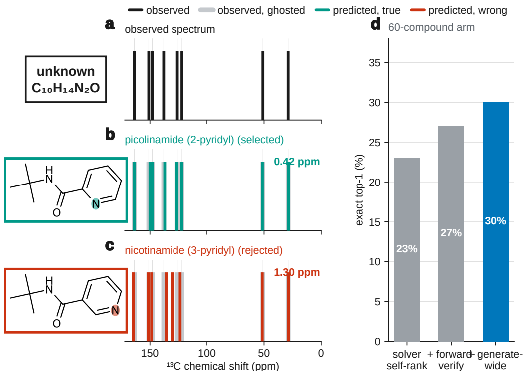
Fig. 5. Forward-verification elucidation. (a–c) Regioisomer pair from the benchmark: picolinamide and nicotinamide are indistinguishable to the inverse task, but forward-predicted ^{13}C sticks separate the true isomer from the alternative (§5.1). (d) Inference ladder on the 60-compound arm (§5.3); the hero bar is generate-wide top-1.
