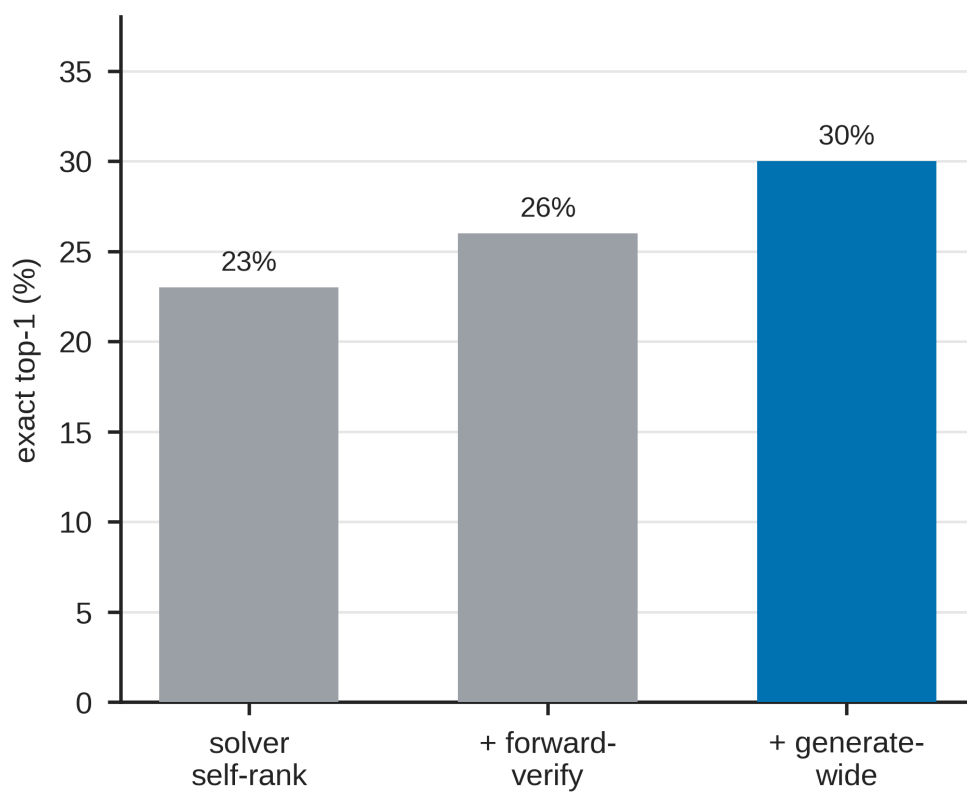
Fig. 5: Forward-verification inference ladder on the same 60 compounds: solver self-ranking \rightarrow + forward-verify \rightarrow + generate-wide (23%/26%/30% top-1).
