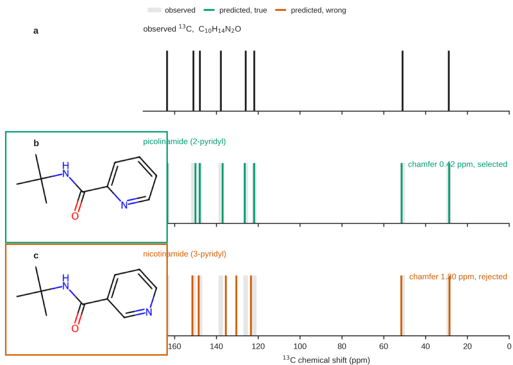
Fig. 4: Forward-verification on a real benchmark regioisomer pair (picolinamide vs nicotinamide): forward-predicted ^{13}\text{C} matches the true isomer (chamfer 0.42 vs 1.30 ppm) — an analog of NMR-crystallography.
