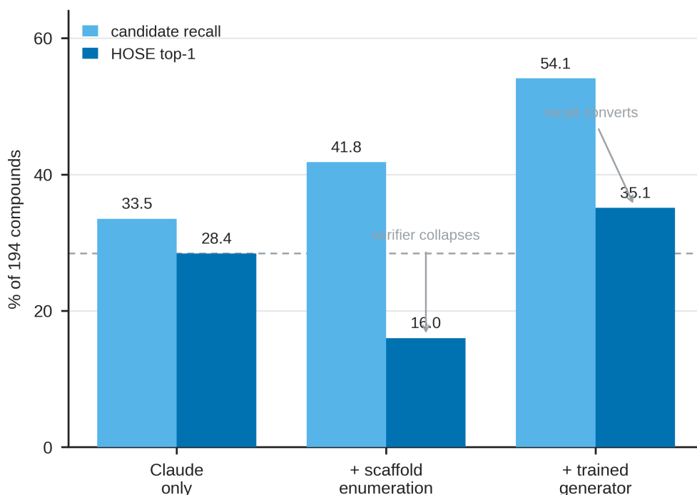
Fig. S5: Trained-generator probe (§5.6; a complement, not part of the training-free protocol). Candidate recall and deterministic-HOSE top-1 on the 194-compound benchmark for Claude / + scaffold enumeration / + trained generator: enumeration’s near-degenerate isomers collapse the verifier (28.4%→16.0%) while the generator’s formula – correct candidates convert (28.4%→35.1%).
