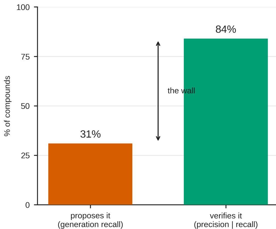
Fig. 1: The diagnosis in one glance: shown a candidate set, the model verifies the true structure 84% of the time it is in the candidate set (conditional on recall, n=19 ; roughly 18 pt above the derangement floor of \$5.5 ), yet the model proposes it for only 31% of compounds ( n=60 ). Recall, not verification, is the wall.
