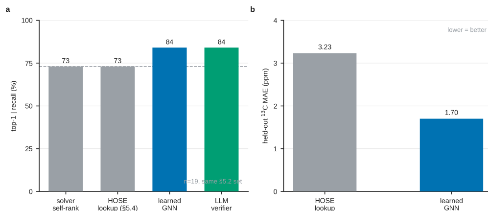
Fig. S6: Learned-verifier probe (§5.7; a complement, not part of the training-free protocol). (A) Conditional-on-recall top-1 (n=19) across four verifiers: a GNN trained on the same nmshiftdb2 data as the HOSE lookup recovers the LLM verifier’s 84% that the lookup (73%) could not. (B) Held-out ^{13}\text{C} MAE — the learned model is roughly 2× sharper (1.70 vs 3.23 ppm).
