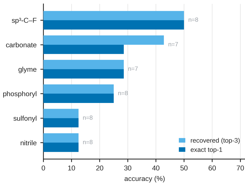
Fig. S4: IRSpectra-Bench-Electrolyte by battery-electrolyte class (n=46): sp 3 -C-F easiest (50%), sulfonyl and nitrile hardest (12%).
