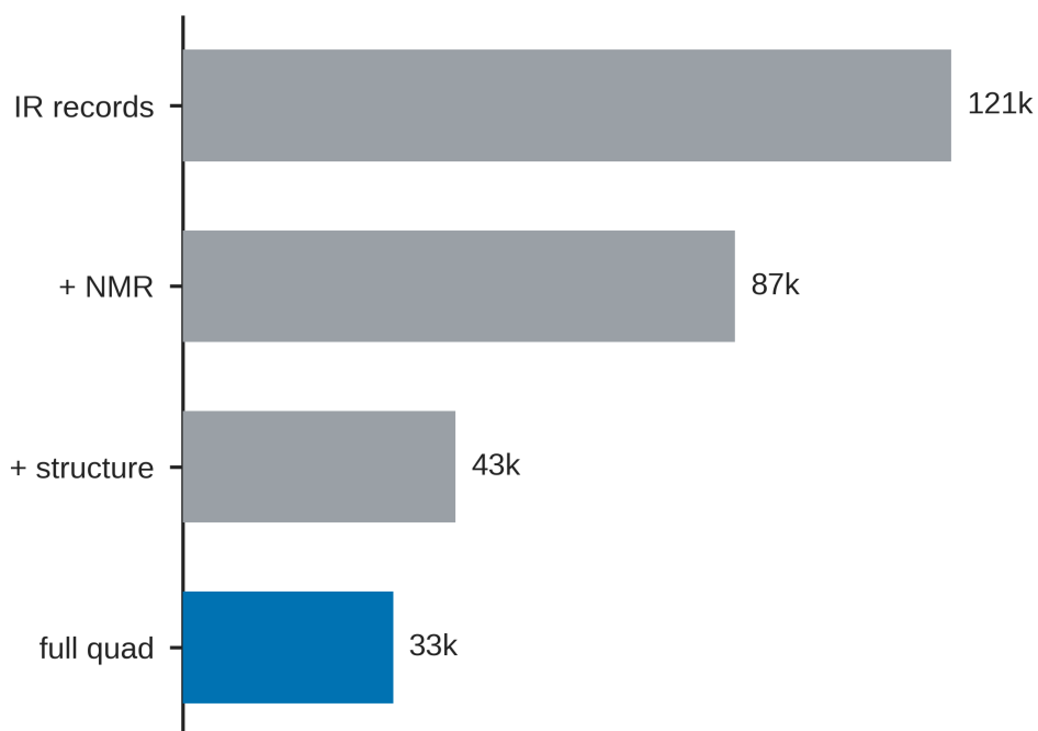
Fig. S2: IRexp composition: IR records, NMR-paired, structure-linked, and full IR+ 1 H+ 13 C+structure quadruples.
