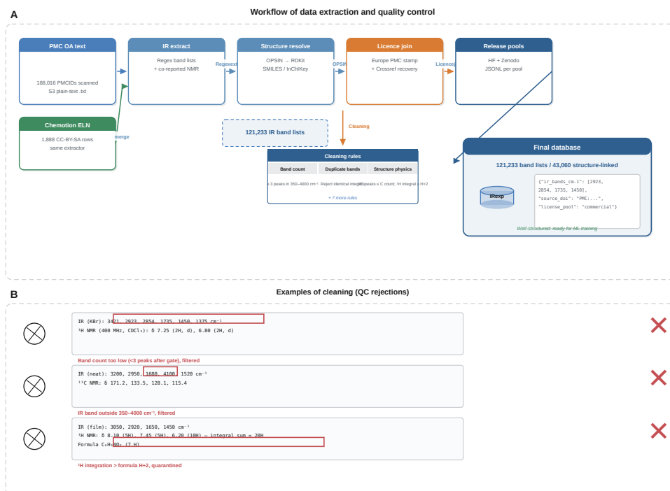
Fig. 2 Workflow of data extraction and examples of cleaning. (A) Construction pipeline: 188,016 PMC Open Access identifiers scanned; deterministic regex extraction of IR band lists and co-reported NMR strings; OPSIN/RDKit structure resolution; Europe PMC licence join with Crossref recovery; segregation into redistribution pools (Hugging Face / Zenodo). Cleaning rules (inset) gate band count, duplicates, and structure–NMR physics. Final release: 121,233 band lists / 43,060 structure-linked. (B) Representative QC rejections (red highlight = failure reason).
