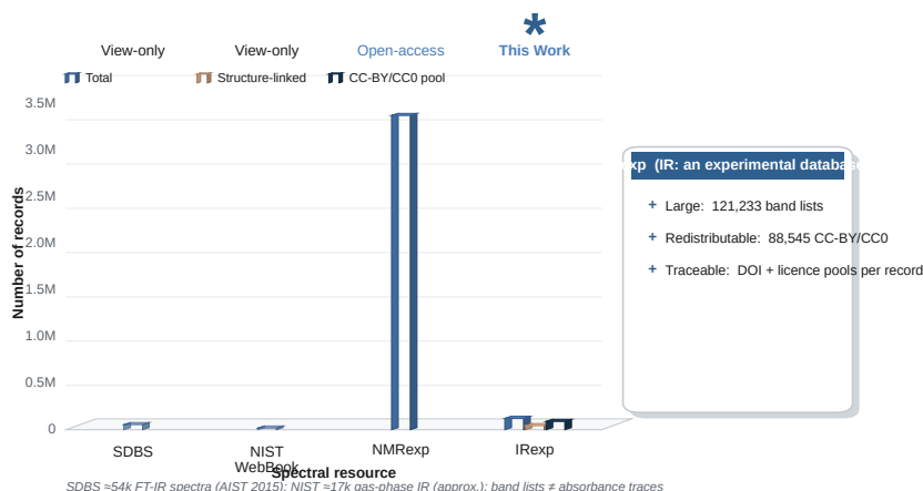
Fig. 1 Summary of major IR and spectral-list resources. IRexp (this work) holds 121,233 experimental band lists ( \text{cm}^{-1} peak positions) with bulk redistribution and per-record licence pools; stacked bars show structure-linked (43,060) and commercial CC-BY/CC0 (88,545) subsets. NMRexp [4] is the modality peer for literature-mined NMR peak lists (3,372,987 records; different object). SDBS FT-IR ( \sim 54,000 digitised absorbance spectra; AIST 2015) and NIST WebBook ( \sim 17,000 gas-phase IR; approximate) are view-only with no bulk export. Sidebar: IRexp scale, redistributable commercial pool, and DOI traceability. Band lists \neq absorbance spectra.
