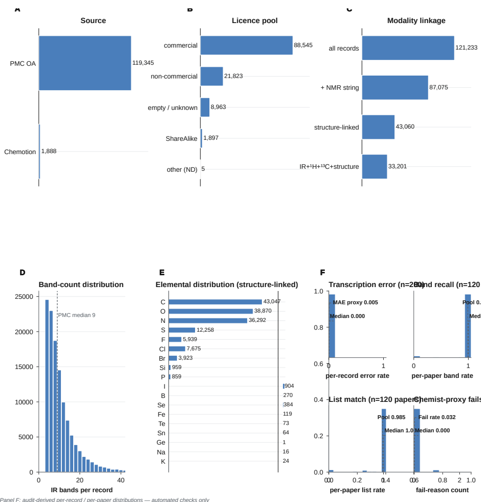
Fig. 3 Data distribution analysis and technical validation of IReXP. (a) Provenance (PMC Open Access Subset vs Chemotion/RADAR4Chem). (b) Licence pools after Europe PMC joins and Crossref empty-licence recovery. (c) Modality linkage cascade to full IR + 1 H + 13 C + structure quadruples (33,201). (d) IR band-count distribution (median 9 bands for PMC rows). (e) Elemental distribution in the structure-linked subset (43,060 records). (f) Audit-derived validation histograms: transcription error per record ( n = 200 ), per-paper band recall and list match ( n = 120 ), and chemist-proxy fail counts ( n = 280 ); dashed elbows mark medians and pool-level rates. All panel (f) checks are automated — not NMRexp-parity human expert audits.
