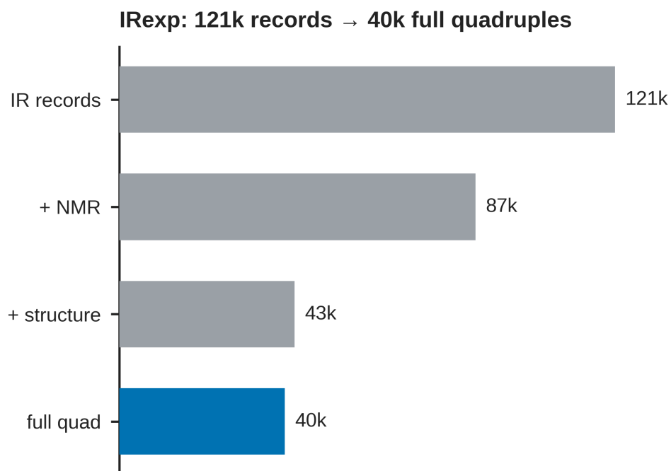
Fig. S2: IRexp composition: IR records, NMR-paired, structure-linked, and full IR+ ^1\text{H} + ^{13}\text{C} +structure quadruples.
