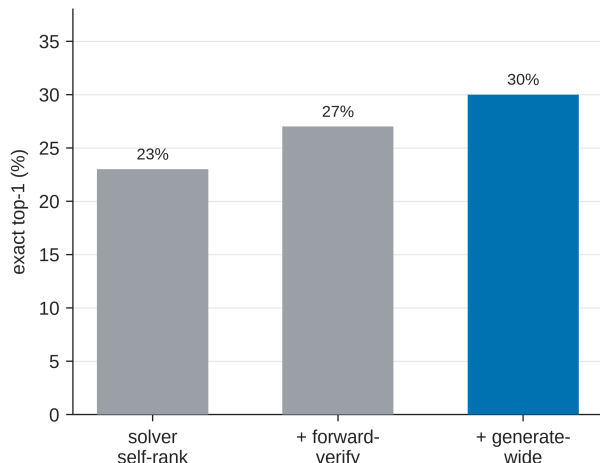
Fig. 6: The forward-verification inference ladder on the 60-compound arm: solver self-ranking \rightarrow + forward-verification \rightarrow + generate-wide, at 23% / 27% / 30% top-1. Each rung is a training-free change to inference alone. The steps are directional rather than individually resolved at this sample size — the paired tests are in §5.3.
