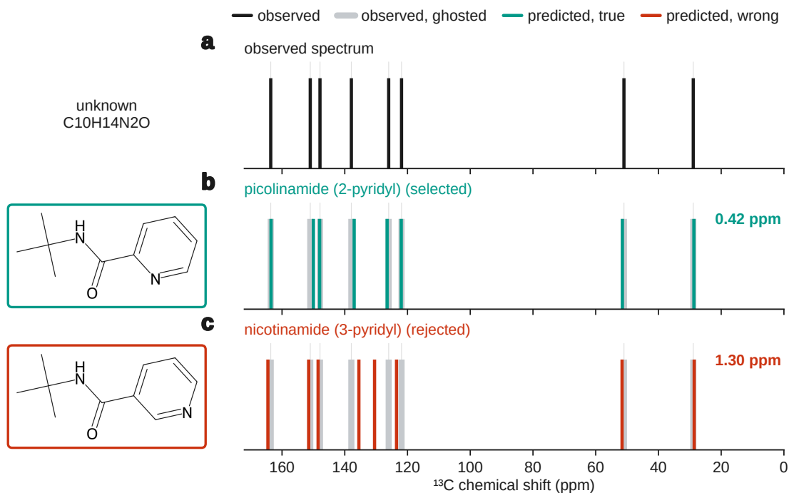
Fig. 6. Forward-verification on a benchmark regioisomer pair: picolinamide and nicotinamide are indistinguishable to the inverse task, but forward-predicted 13 C sticks separate the true isomer from the alternative (§5.1).
