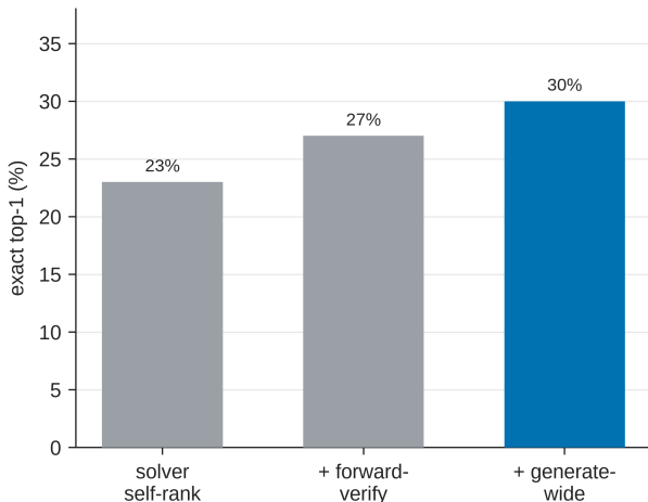
Fig. 6: The forward-verification inference ladder on the 60-compound arm: solver self-ranking → + forward-verification → + generate-wide, at 23% / 27% / 30% top-1. Each rung is a training-free change to inference alone, directional rather than individually resolved at this sample size (§5.3).
