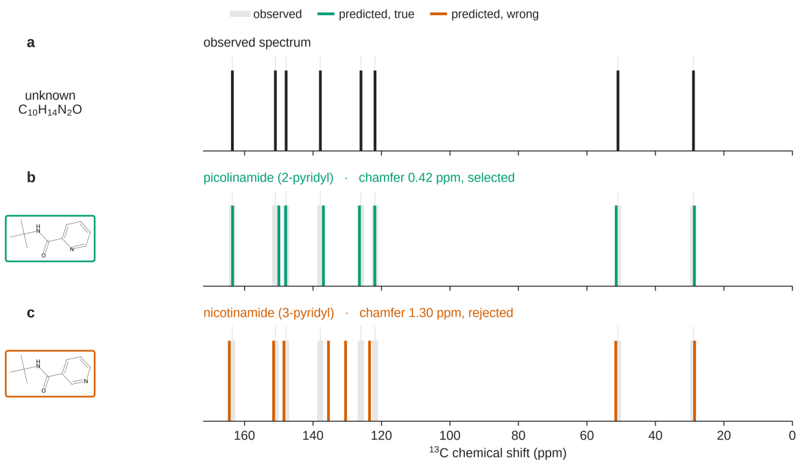
Fig. 5: Forward-verification on a benchmark regioisomer pair: picolinamide and nicotinamide are indistinguishable to the inverse task, but the true isomer’s forward-predicted ^{13}\text{C} spectrum matches the observed one at a chamfer of 0.42 ppm against 1.30 ppm for the alternative (§5.1).
