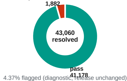
D Structure-NMR quarantine (n=43,060)
