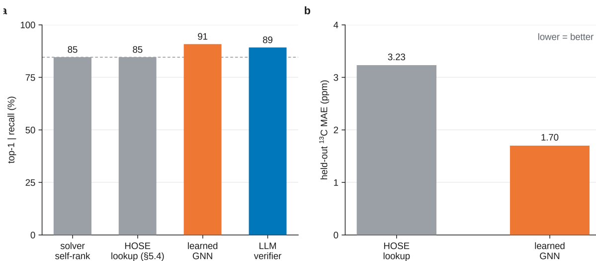
Fig. S6. Learned-verifier probe (§5.4; a complement, not part of the training-free protocol). (a) Conditional-on-recall top-1 over the whole benchmark (n=65) across four verifiers: a GNN trained on the same nmr-shiftdb2 data as the HOSE lookup reaches the LLM verifier’s level (91% against 89%) where the lookup (85%) does not move off the solver’s own ranking. (b) Held-out ^{13}\text{C} MAE — the learned model is roughly 2× sharper (1.70 vs 3.23 ppm).
