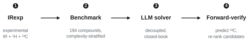
Fig. S1. Study design: open multimodal data (IRexp) → blind, complexity-stratified benchmark → decoupled blind solving → forward-verification re-ranking; training-free core pipeline.
