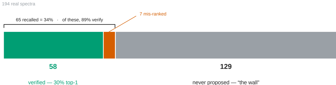
Fig. 1. All 194 benchmark compounds as a single part-to-whole bar. The true structure is verified top-1 for 58 (green), recalled but mis-ranked for 7 (vermillion), and never proposed for 129 (grey): the wall , 66% of the bar. Generation recall (the fraction of compounds whose true structure appears anywhere in the solver’s candidate list) is 65/194 = 34\% . Of those 65, forward-verification then ranks 58 first: verification precision (conditional on recall) is 58/65 = 89\% . Their product is the 30% end-to-end top-1. The two rates have different denominators and are not differenced.
