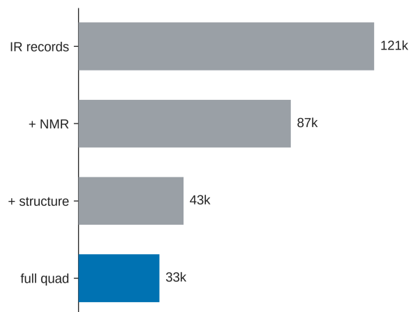
Fig. S2. IReXP composition: IR records, NMR-paired, structure-linked, and full IR+ 1 H+ 13 C+structure quadruples.
