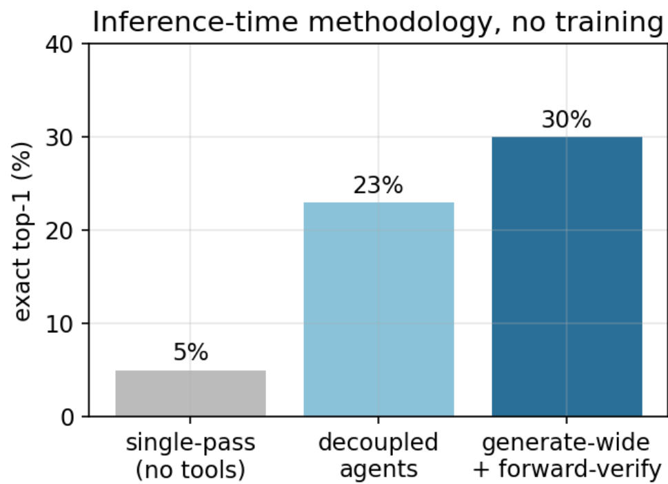
Fig. 8: Inference-time methodology ladder: single-pass \rightarrow decoupled agents \rightarrow generate-wide + forward-verify (5%/23%/30%).
