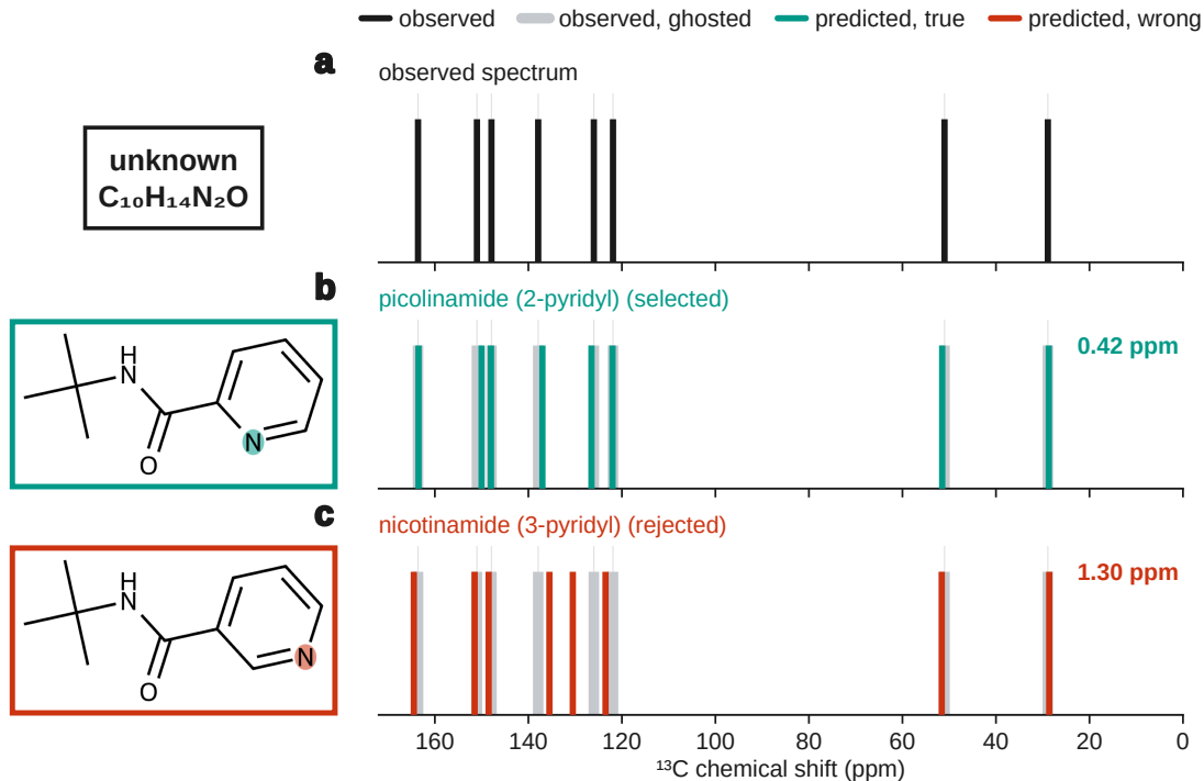
Fig. 5. Forward-verification on a benchmark regioisomer pair: picolinamide and nicotinamide are indistinguishable to the inverse task, but forward-predicted 13 C sticks separate the true isomer from the alternative (§5.1).
