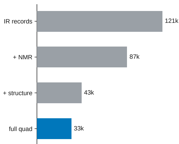
Fig. S2. IRexp composition: IR records, NMR-paired, structure-linked, and full IR+ ^1\text{H} + ^{13}\text{C} +structure quadruples.
