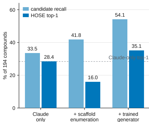
Fig. S5. Trained-generator probe (§5.6; a complement, not part of the training-free protocol). Candidate recall and deterministic-HOSE top-1 for Claude-only, + scaffold enumeration, and + trained generator on the 194-compound benchmark.
