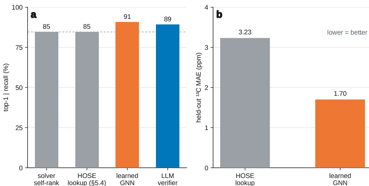
Fig. S6. Learned-verifier probe (§5.4; a complement, not part of the training-free protocol). (a) Conditional-on-recall top-1 over the whole benchmark (n=65) across four verifiers. (b) Held-out 13 C MAE (lower is better).
