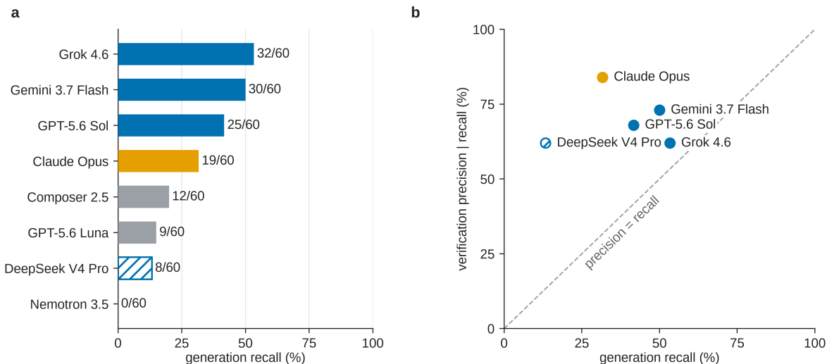
Fig. 5. Cross-vendor decomposition on the 60-compound arm: generation recall vs verification precision (§4.7).
