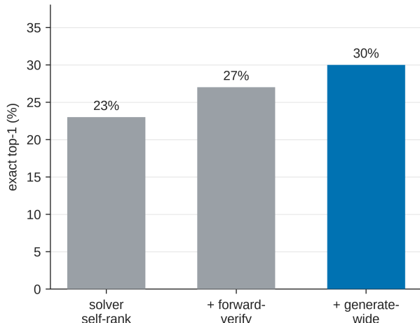
Fig. 7. Forward-verification inference ladder on the 60-compound arm: 23% / 27% / 30% top-1 (§5.3).
