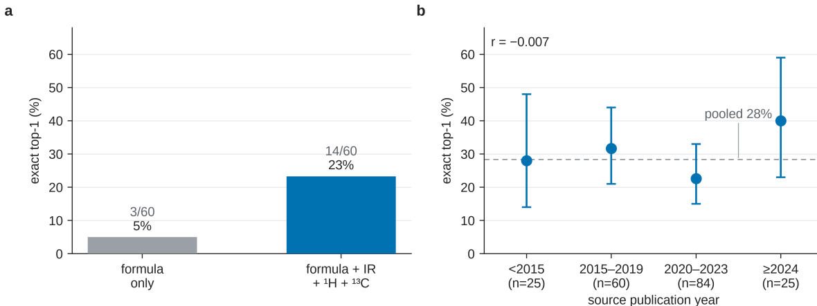
Fig. 4. Two contamination controls. (a) Formula-only vs full modality on 60 compounds. (b) Accuracy vs source-paper year (n=194).
