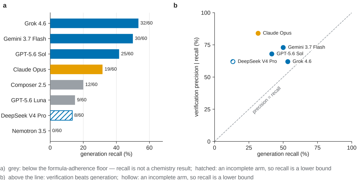
Fig. 5. Every model measured on the 60-compound arm. (a) Generation recall, each model at the candidate budget it used: 3.00 candidates per compound for all but ours (2.20) and Composer (2.82). That axis therefore favours the models that always returned three. Grey marks models below the formula-adherence floor, whose recall is not a chemistry result. (b) The claim itself: verification precision against generation recall, with the diagonal. Every model sits above the line, so verification is better than generation for all four families; hollow marks an incomplete arm, where recall is a lower bound. The four Claude models of §4.4 are deliberately absent: they ran a different 24-compound subset, and putting them here would imply a comparison that was never made.
