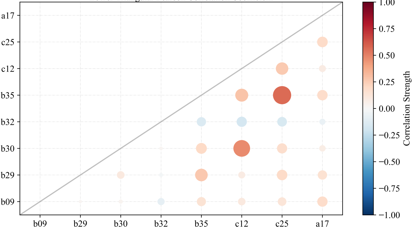
Lower Triangular Pearson Correlation Coefficient
