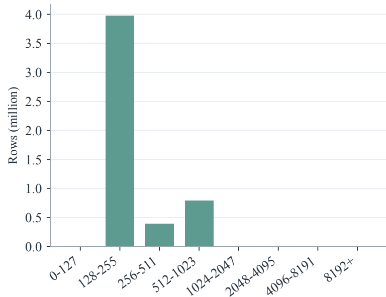
Sequence length bins
