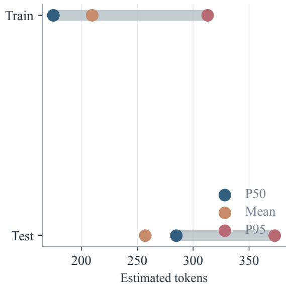
Token cost profile
