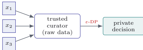
Central model: privatize the output
