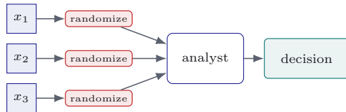
Local model: privatize before sharing
