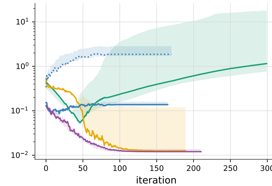
S4: L-shaped reentrant corner
