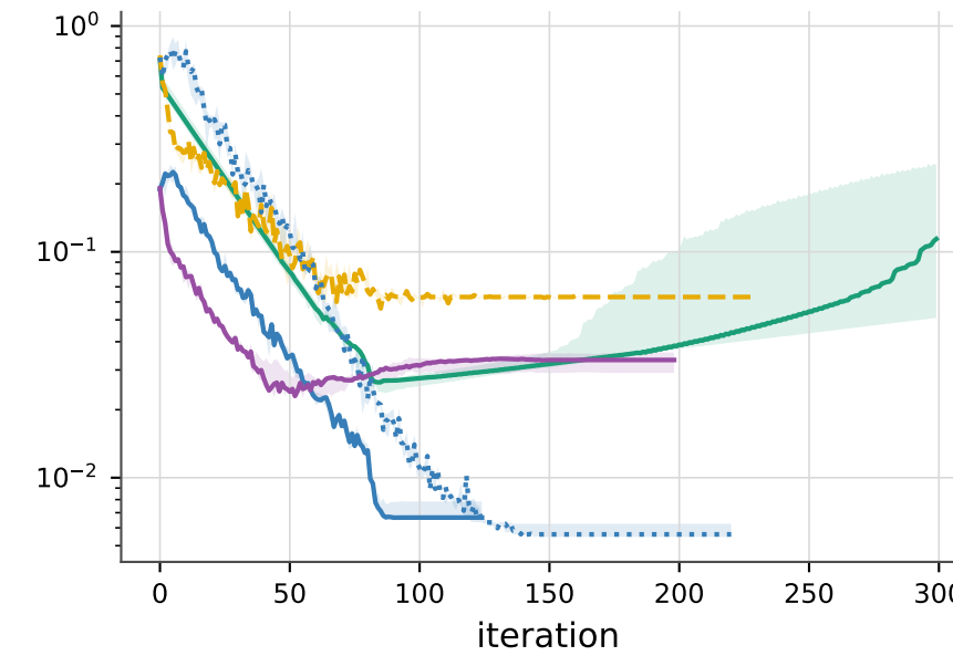
S3: line source / kink
