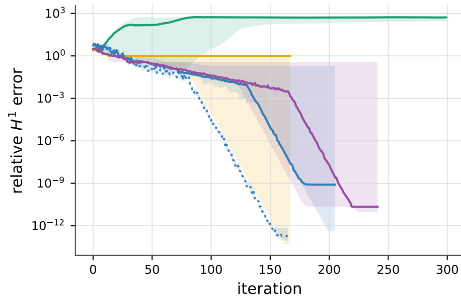
S1: multiscale A-Laplacian
