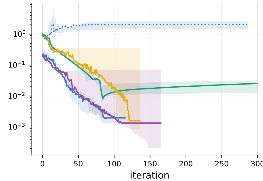
S2: discontinuous forcing
