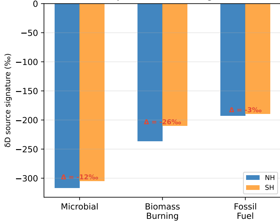
E. Hemispheric \delta\text{D} source signatures
